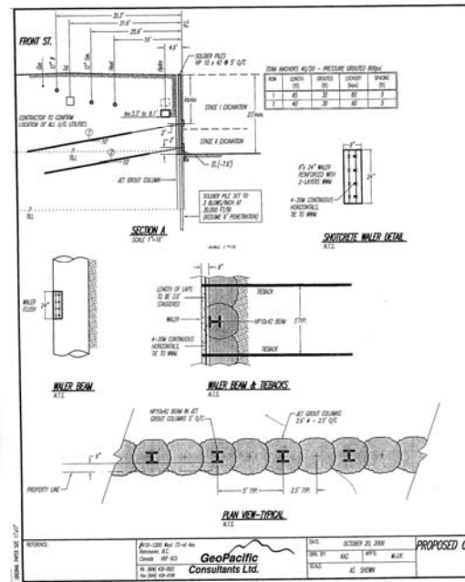
Figure2: Typical section and plan of the jet-grouted wall
